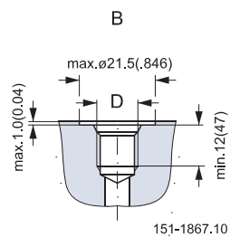
B: UNF main ports D: \frac{7}{16} - 20 UNF O-ring boss port
