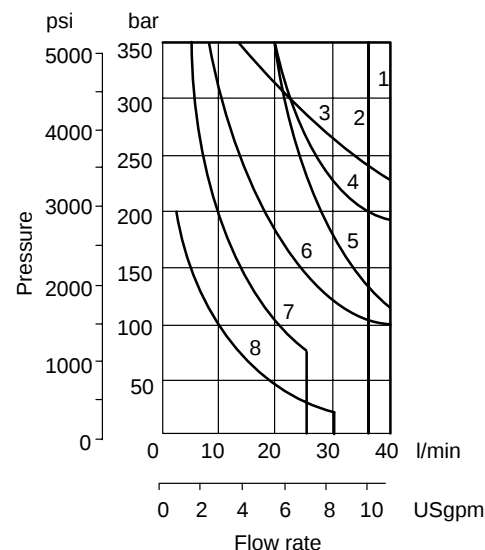
Graph 2 AC solenoid valves with – Dual frequency coils operating at 60 Hz – Single frequency (50 Hz) coils operating at 50 Hz
